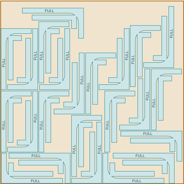
LAYER 4 - UNKNOWN courses 1-2 23 forms
