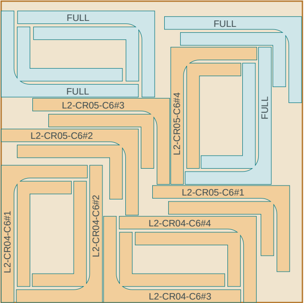
LAYER 1 - L2 course 6 12 forms
