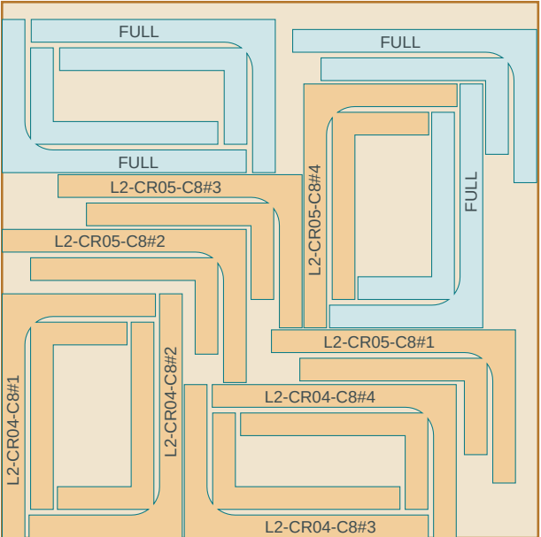
LAYER 1 - L2 course 8
