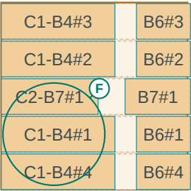
LAYER 9 - L1 courses 1, 2, 3, 5, 7
