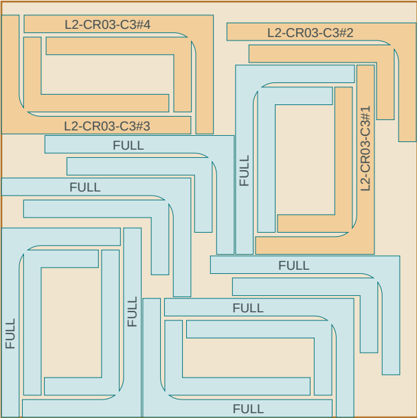
LAYER 4 - L2 course 3 12 forms
