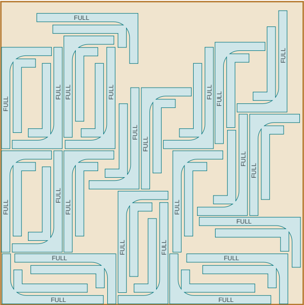
LAYER 3 - UNKNOWN courses 2-3 23 forms
