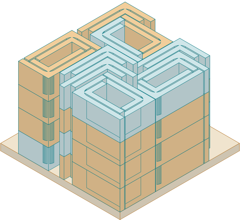
ISOMETRIC 4 layers, built bottom up
