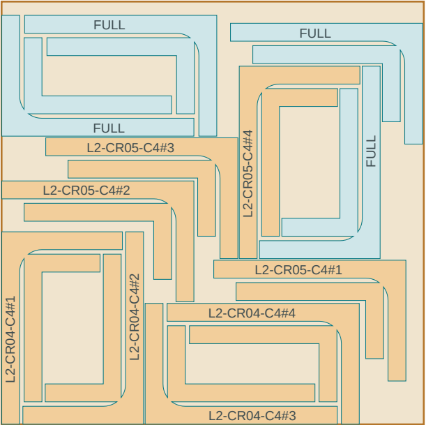
LAYER 1 - L2 course 4 12 forms
