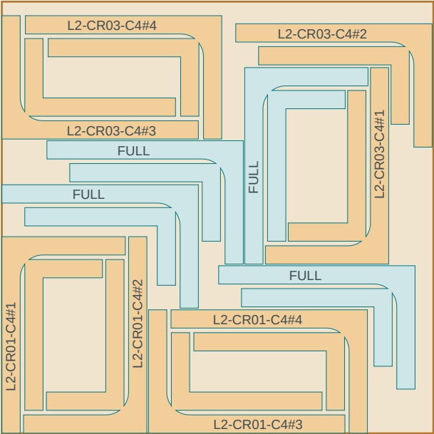
LAYER 2 - L2 course 4 12 forms
