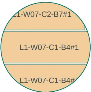
DETAIL F layer 8, 2x
