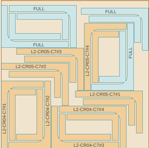
LAYER 3 - L2 course 7
