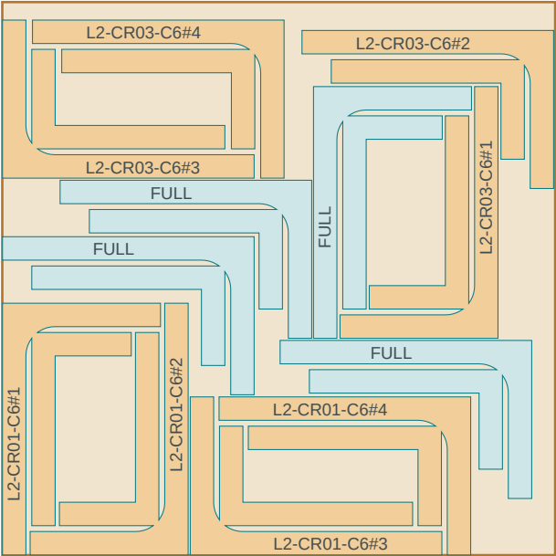
LAYER 2 - L2 course 6 12 forms
