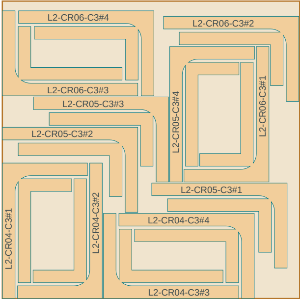
LAYER 3 - L2 course 3 12 forms
