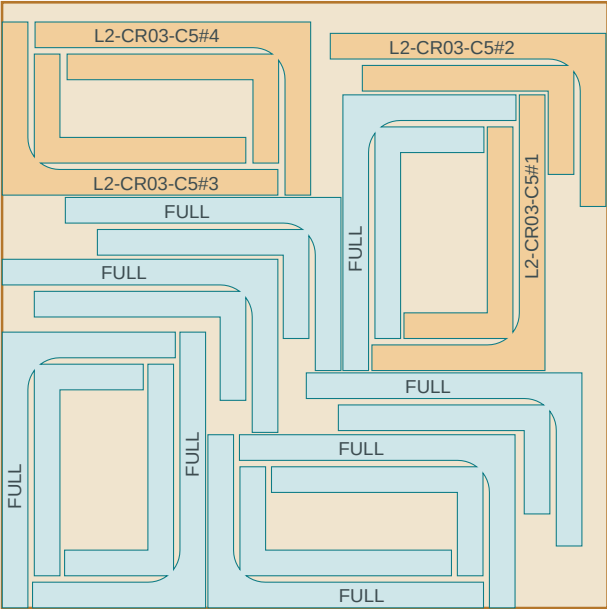
LAYER 4 - L2 course 5 12 forms
