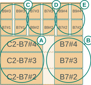
LAYER 9 - L1 courses 1, 2, 3, 5, 7
