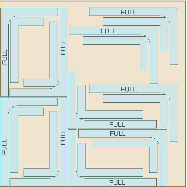
LAYER 1 - L1 courses 3-4 10 forms
